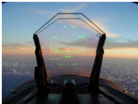
Heads up display (HUD) in an F/A-18 Hornet (Note HUD Camera Periscope at bottom in the center).
